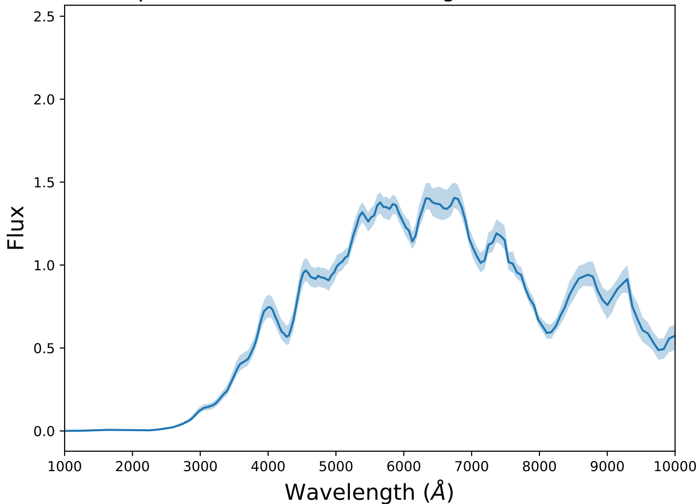
Spectrum 7 for transient 91bg-like at z=1.51
